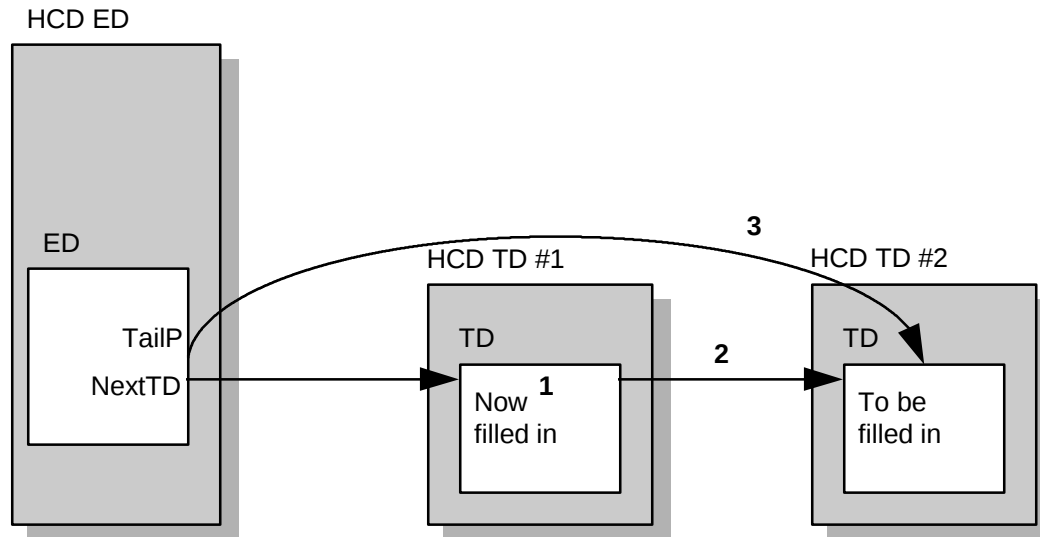
Figure 5-7: Adding a Transfer Descriptor to a Queue
