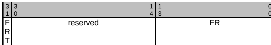
Figure 7-15: HcFmRemaining Register
