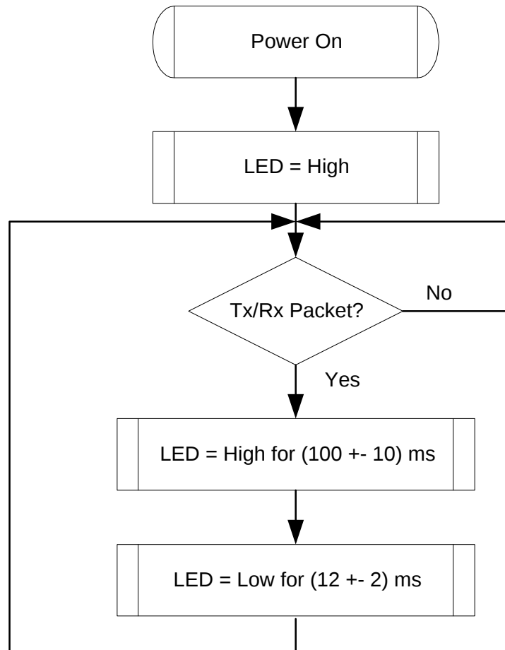
Figure 5. TX/RX LED
