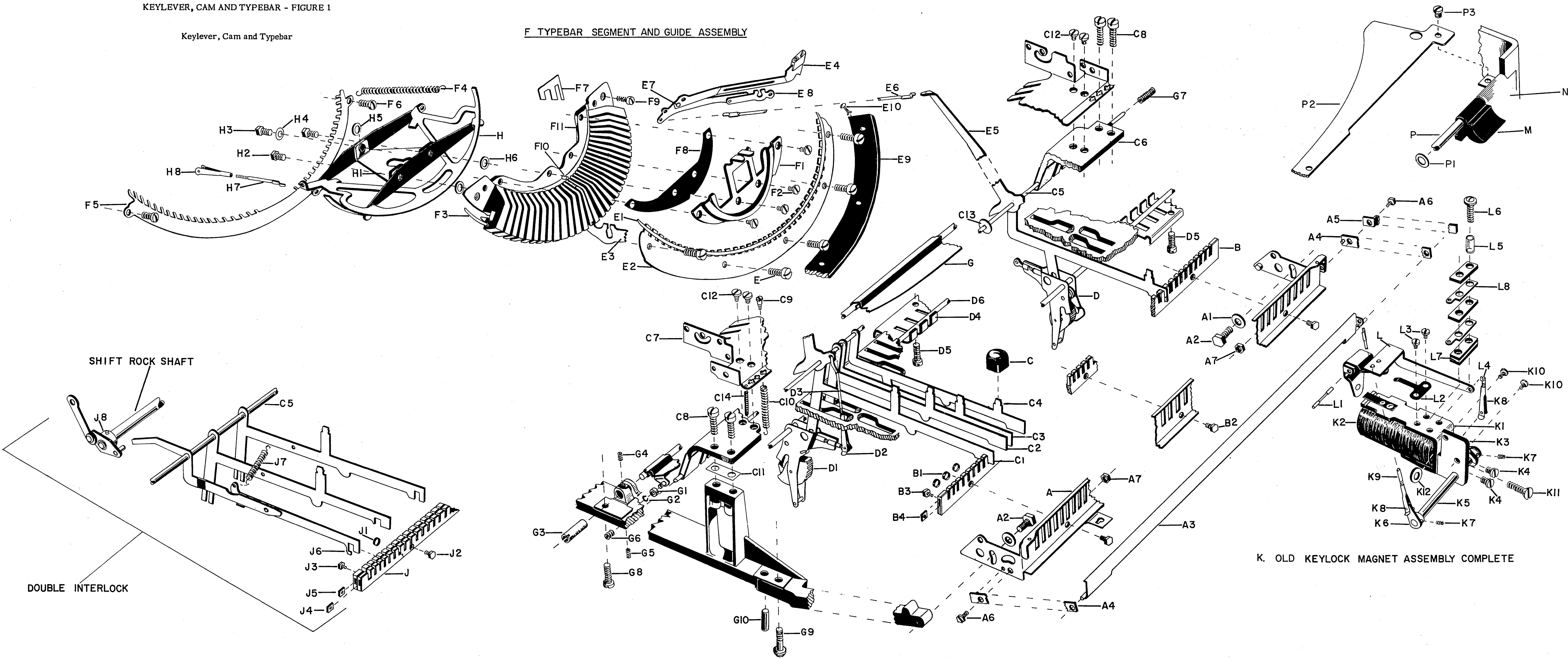
KEYLEVER, CAM AND TYPEBAR - FIGURE 1
