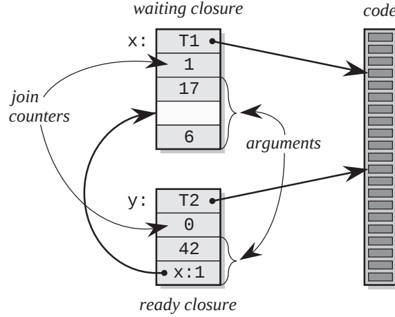
Figure 2: The closure data structure.
