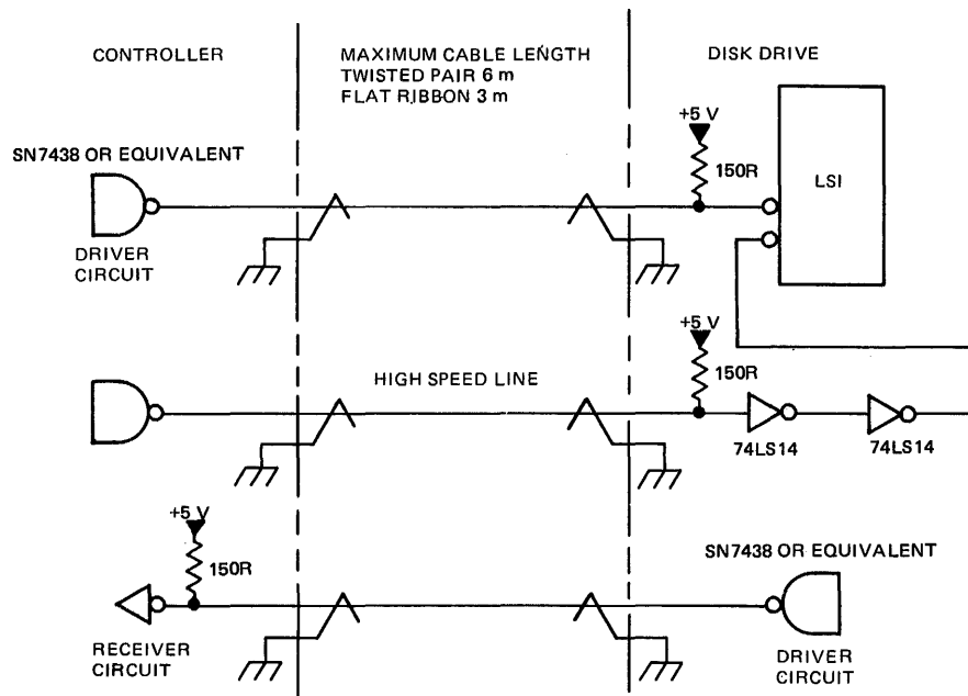
Figure 3-1 Driver/Receiver Circuits
