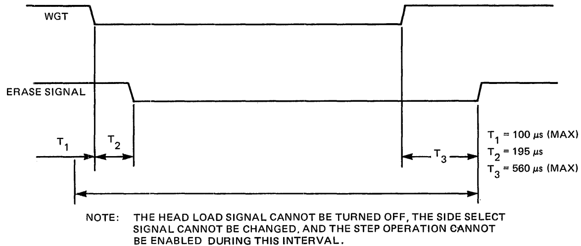
Figure 3-4 WGT Timing
