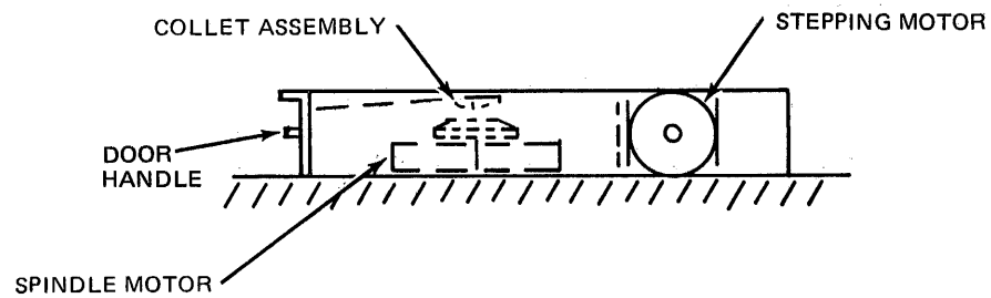
Figure 2-4 Horizontal Installation
