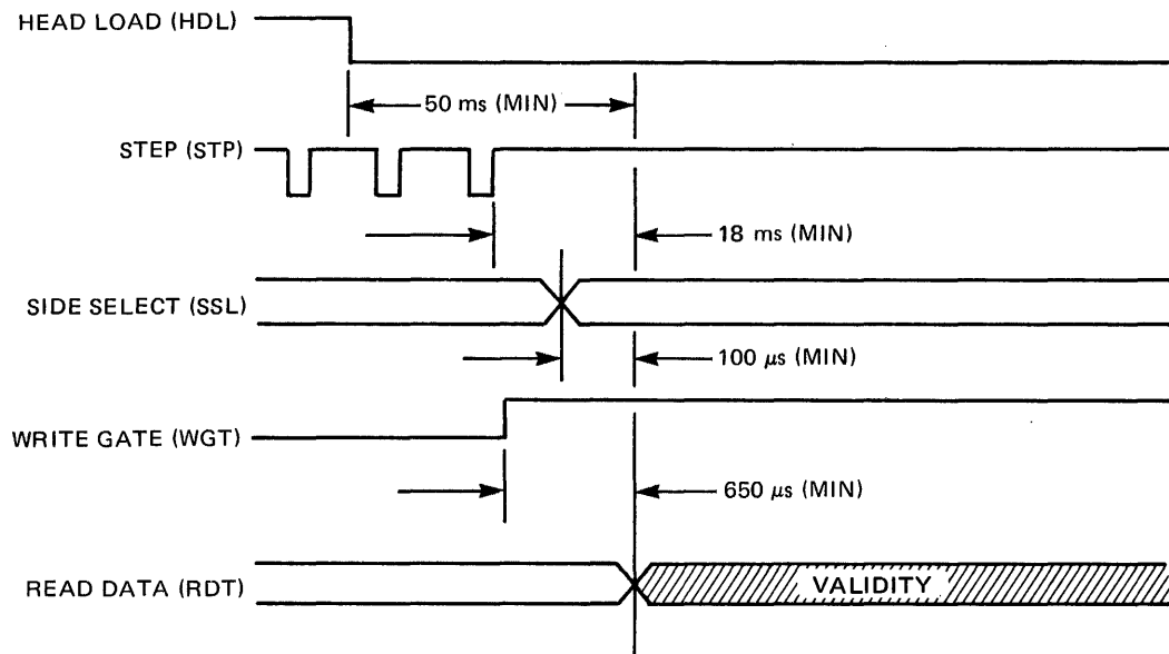
Figure 3-13 Read Timing
