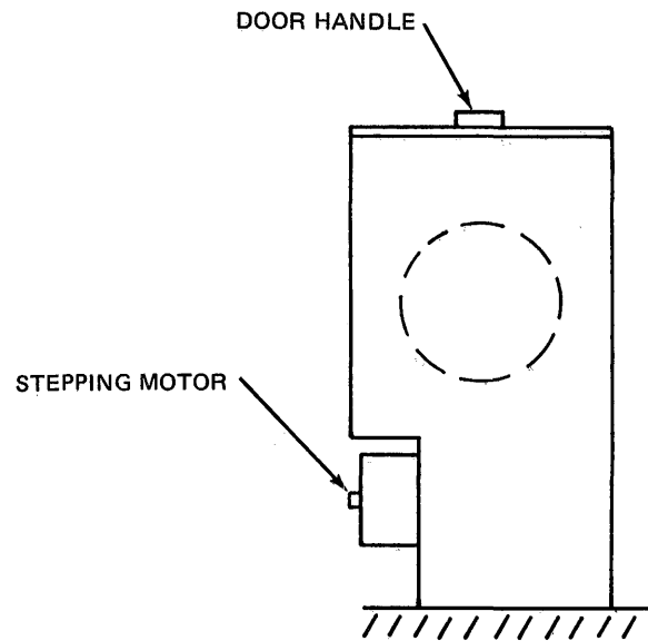
Figure 2-5 On-End Installation
