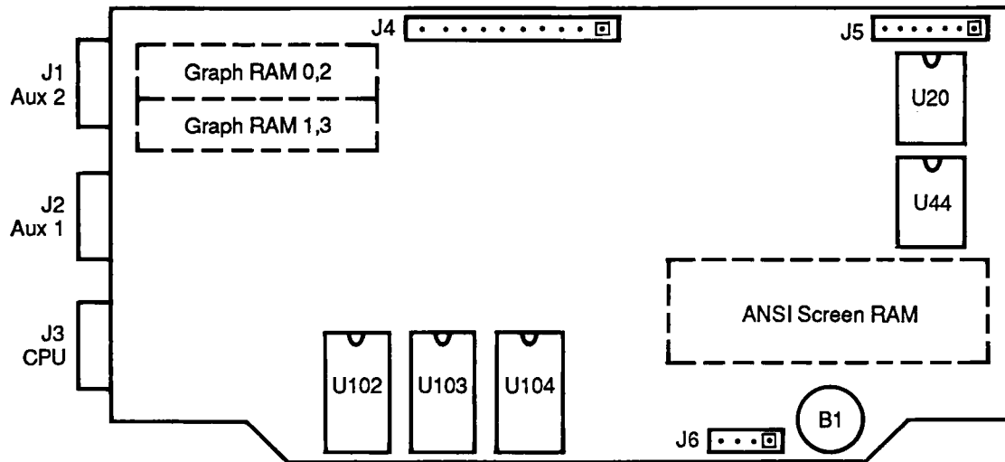
Figure 1. Board Layout
