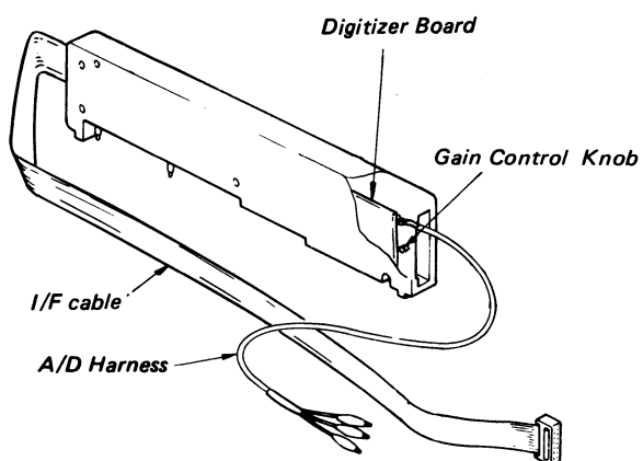
Fig. 2-7 Configuration
