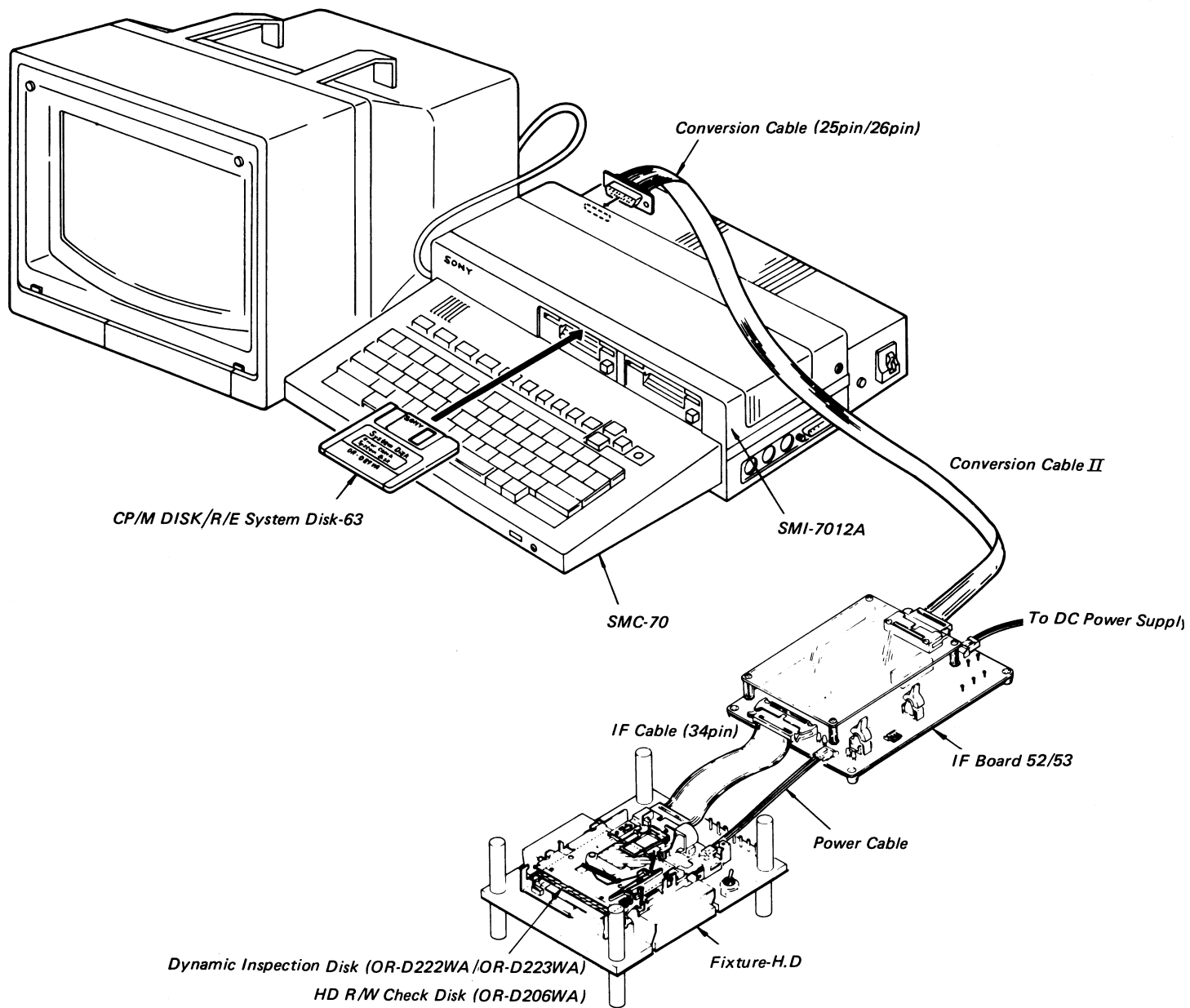
Fig. 2-12 System Configuration for Drive Test (2M Byte mode)
