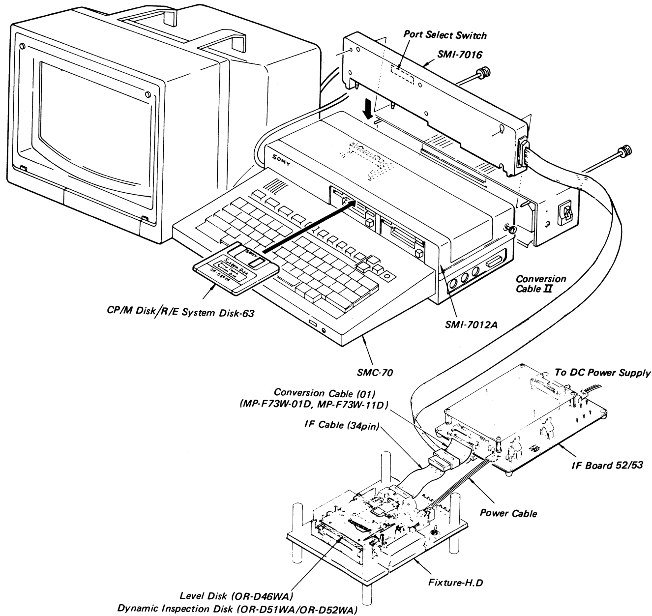
Fig. 2-11 System Configuration for Drive Test (1M Byte mode)
