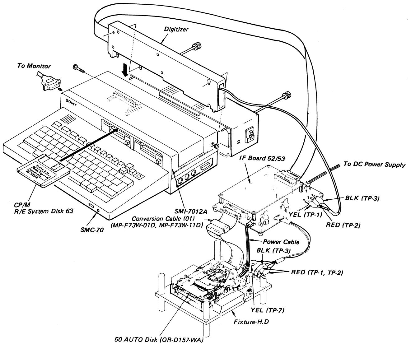
Fig. 2-13 System Configuration for Radial Alignment
