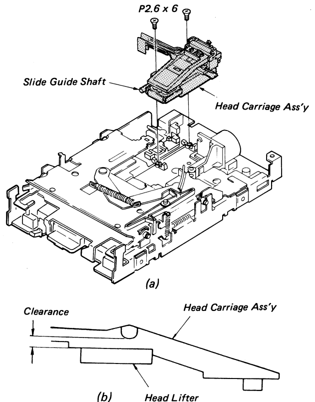
Fig. 4-7 Head Carriage Ass'y Replacement
