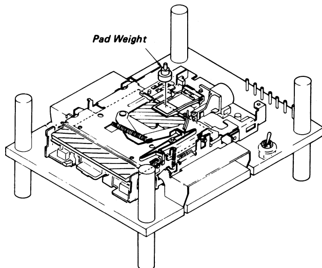
Fig. 5-2 Head Compliance Measurement
