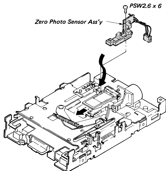
Fig. 4-5 Zero Photo Sensor Ass'y Replacement
