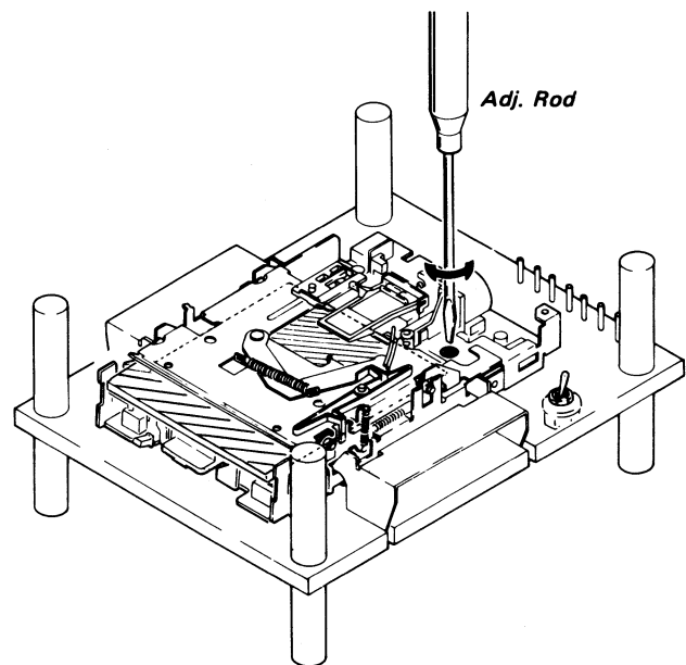
Fig. 5-3 Index Phase Adjustment
