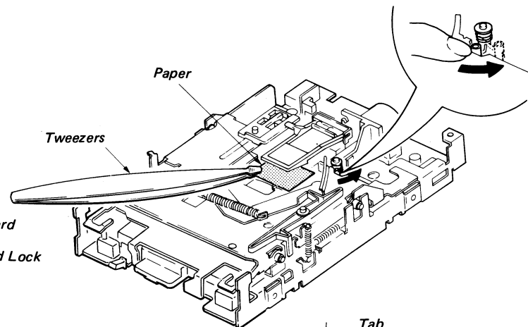
Fig. 4-4 (a) Setting to Disk-In Mode
