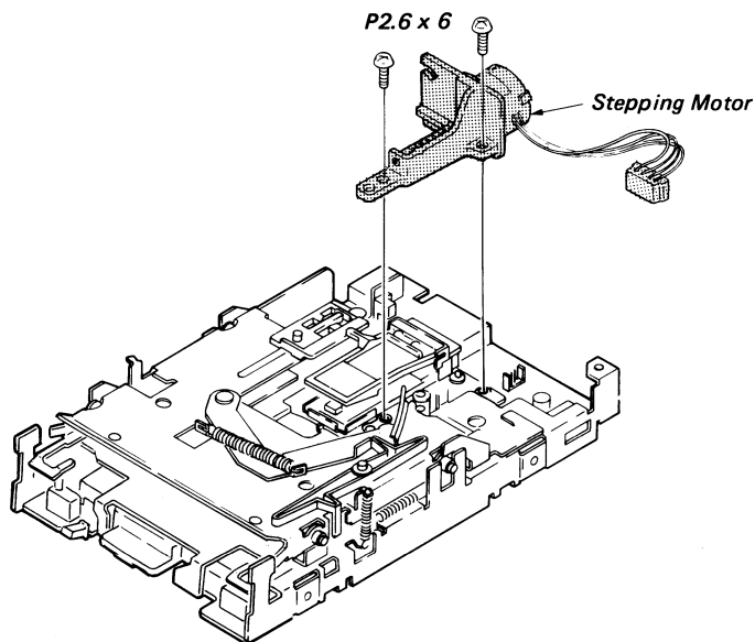
Fig. 4-8 Stepping Motor Replacement
