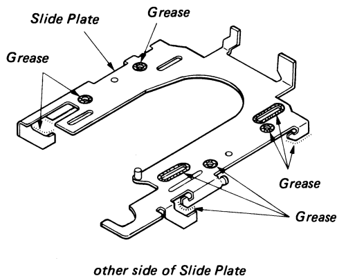
Fig. 4-6 (b) Grease Application Location
