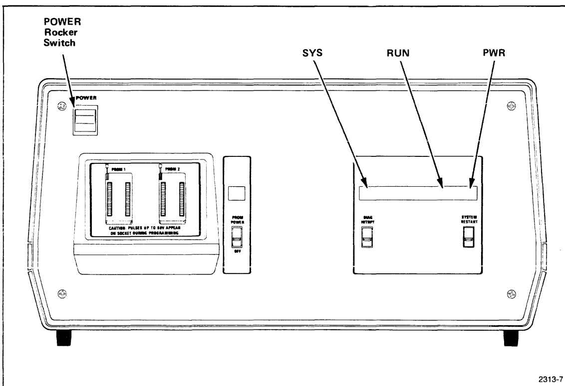
Fig. 2-6. 8002 \mu PROCESSOR LAB Front Panel.
