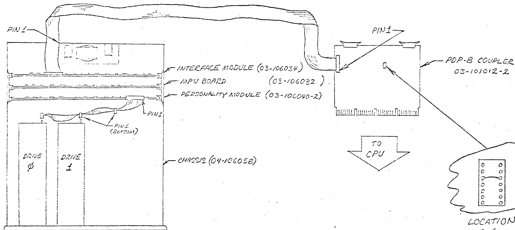
TOP VIEW
