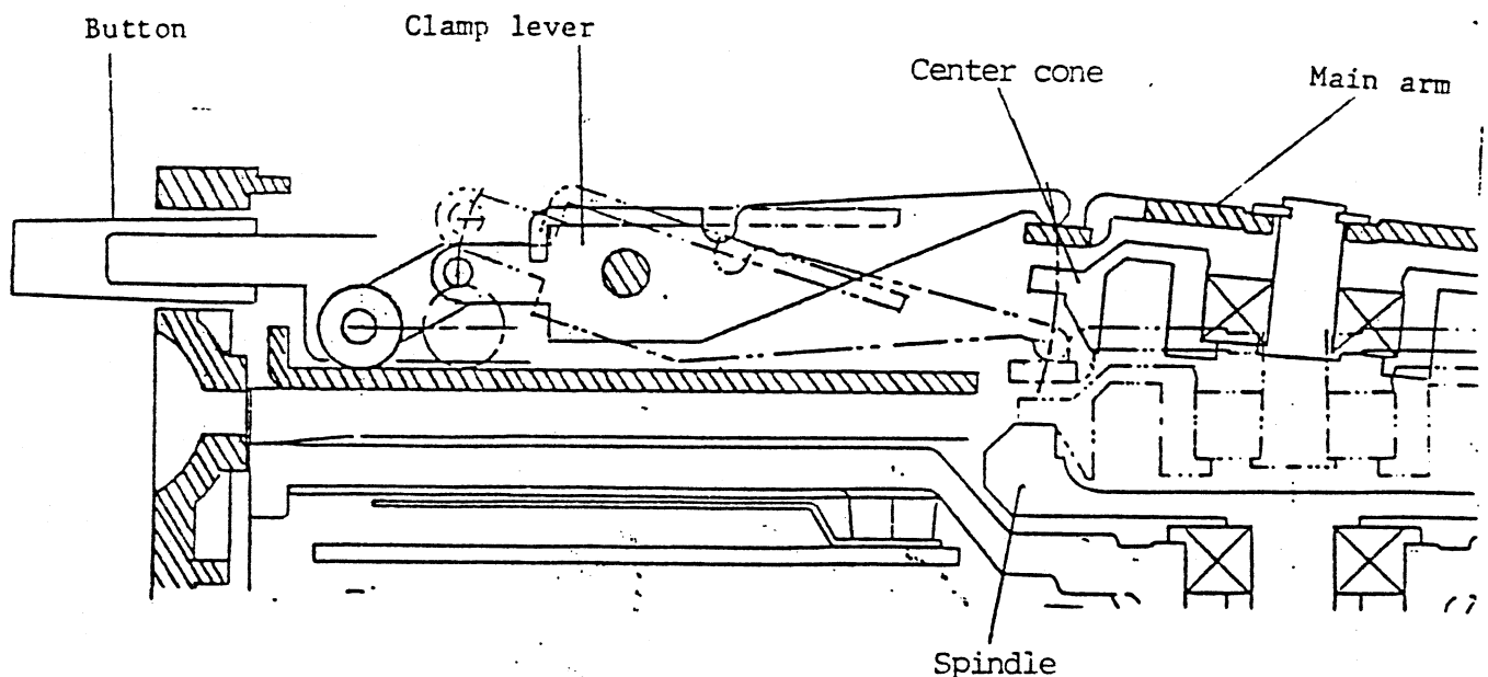
Fig. 3-3 Spindle feature
