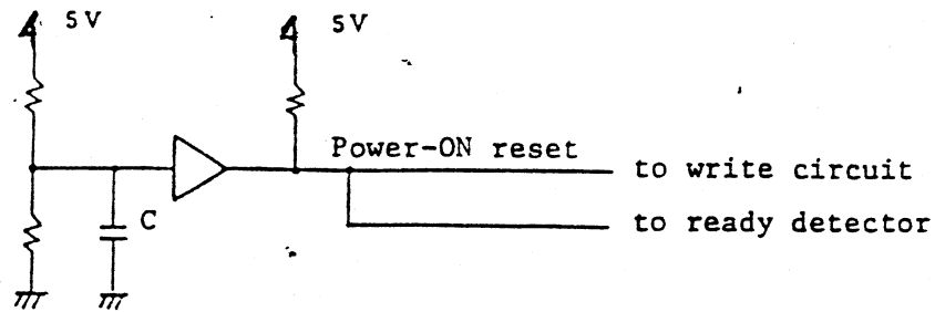
Fig. 3-33 Power-ON reset circuit
