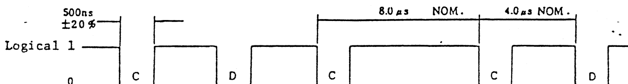
Fig. 2-5 READ DATA (FM)
