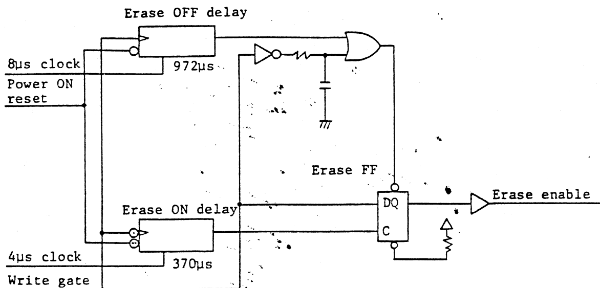
Fig. 3-23 Erase delay circuit (equivalent)
