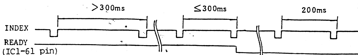
Fig. 3-17 Ready timing
