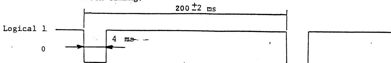
Fig. 2-4 Index timing
