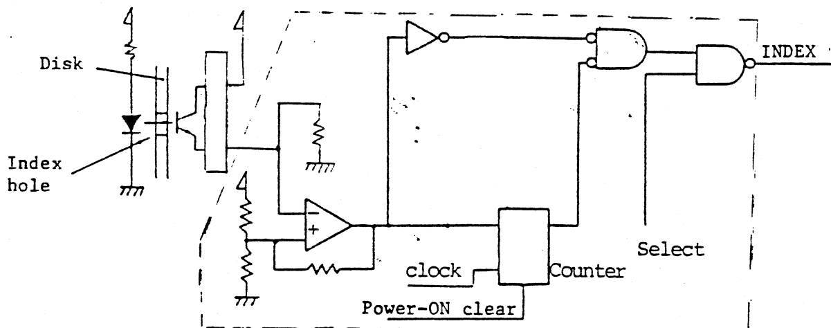
Fig. 3-16 Index detection circuit
